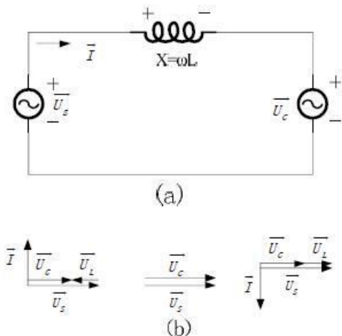
Fig. 2 (a) Equivalent circuit of single phase STATCOM. (b) Vector graphics of equivalent circuit
