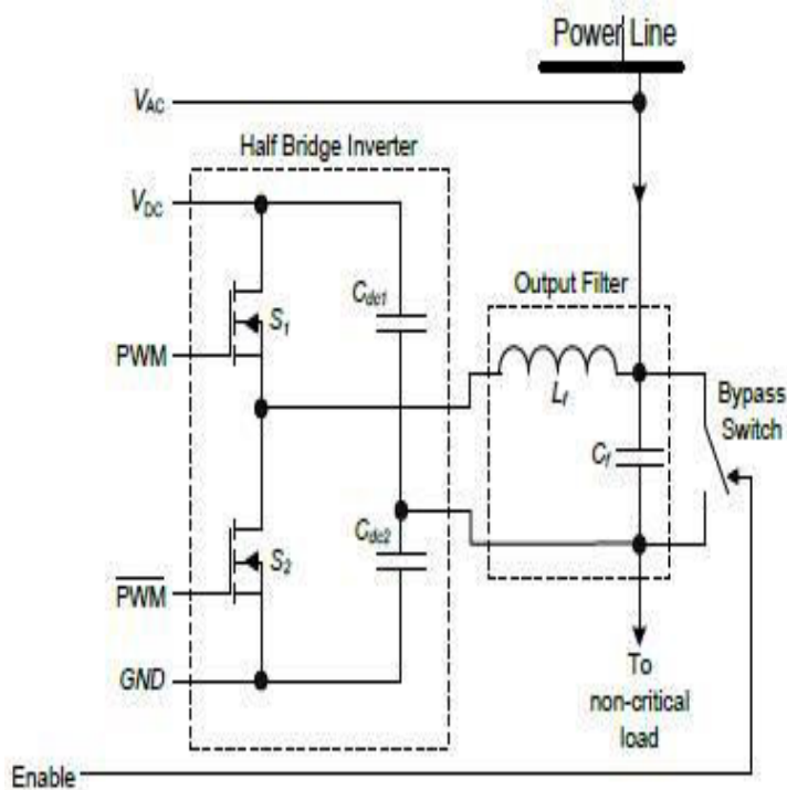
Fig. 4: Schematic of a single phase half bridge power inverter
