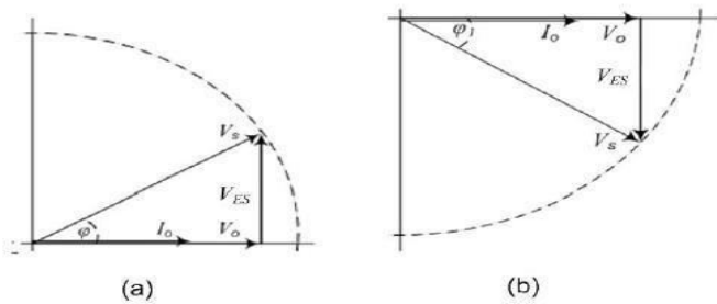
Fig. 5: Phasor diagrams for inductive and capacitive modes of operation of an ES
