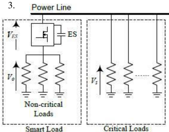
Fig. 3: Smart loads and critical loads in future smart grids
