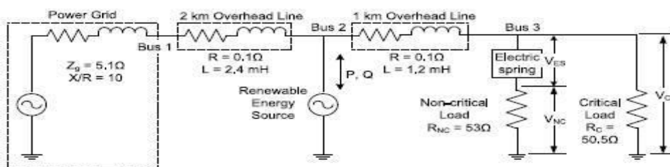
Fig. 7: Simulation set-up with an intermittent source and an equivalent power grid.
