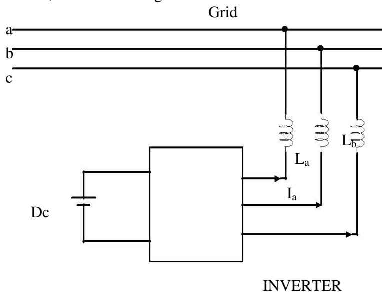
Fig. 1: Voltage bridge topological structure
