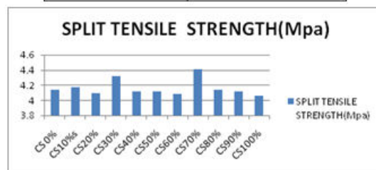
Fig. 4.2 Splitting tensile strength of mixes for 28 days
