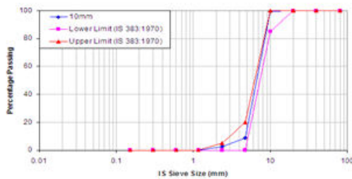
Fig. 3.2 Grading curve of 10 mm coarse aggregate
