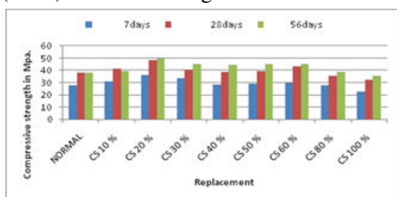
Fig 4.1 compressive strength
