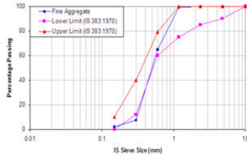
Fig. 3.3 Grading curve of fine aggregate
