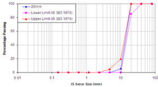
Fig. 3.1 Grading curve of 20 mm coarse aggregate
