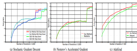
Fig. Fig. 1: CIFAR data set: accuracy-showing plots (Figures 1a-1c) contrasting SGD, NAG and AdaGrad, each with our layer-wise adaptive learning speeds. We display results for the SGD plot both
