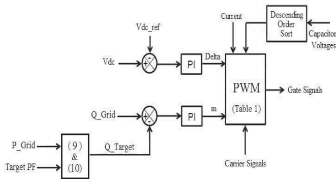
Fig. 3. Schematic of the proposed controller system.
