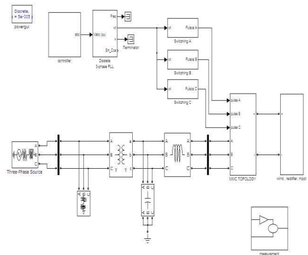
Fig. 5. Matlab/simulink model of the proposed method
