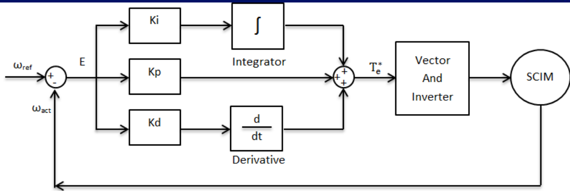
Figure 4: PID controller block diagram.
