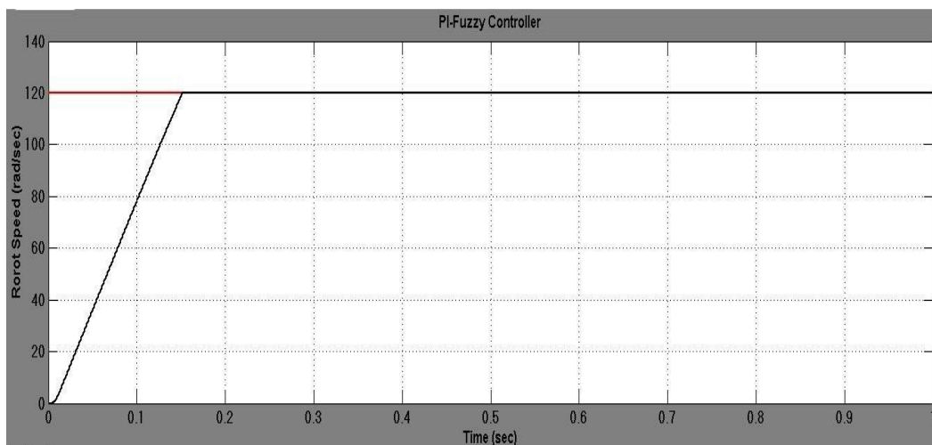
Figure 9: Speed response curve of SCIM at 100 N.m load torque and 120 rad/sec using PI controller
