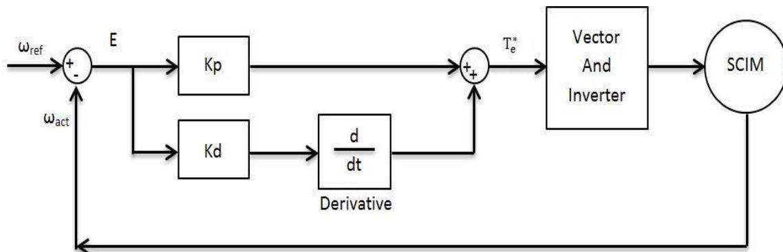
Figure 3: PD controller block diagram.
