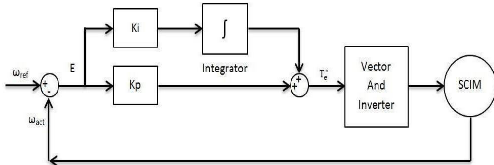
Figure 2: PI controller block diagram.
