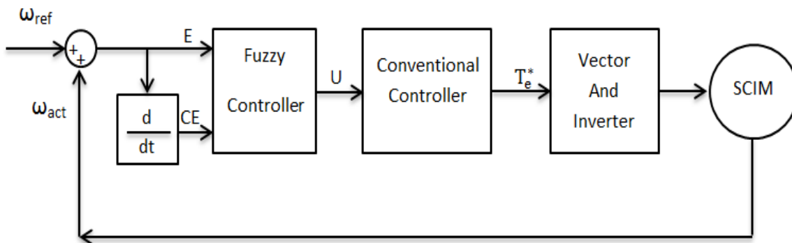
Figure 6: Proposed hybrid controller that combines fuzzy logic controller with conventional controller to drive SCIM
