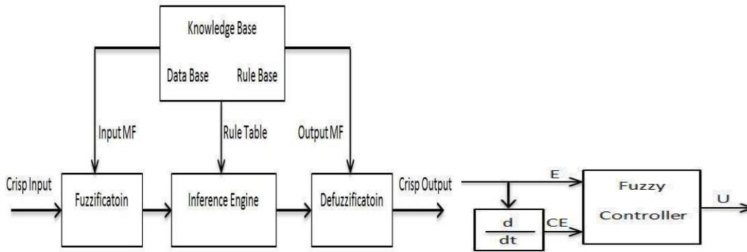
Figure 5: Basic structure of fuzzy logic controller. Fuzzy control system
