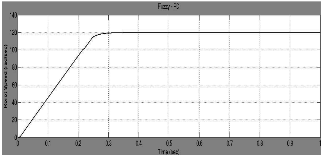
Figure 11: Speed response curve of SCIM at 100 N.m load torque and 120 rad/sec using PD-Fuzzy controller
