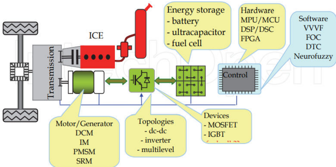
Figure 1: MAJOR COMPONENTS OF HYBRID ELECTRIC VEHICLE
