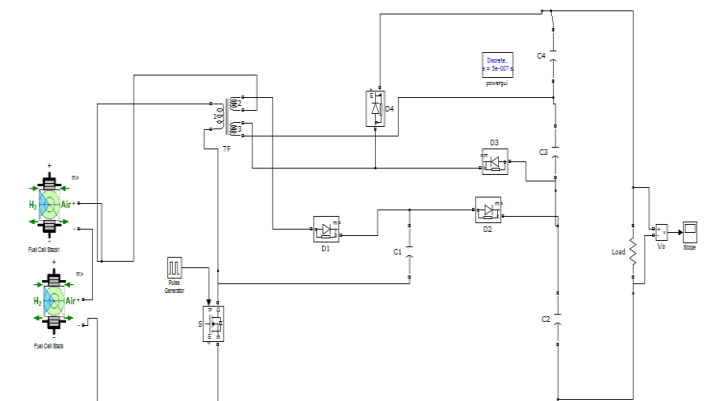
Fig.13.Matlab/Simulation model of high step up Converter with fuel cell.
