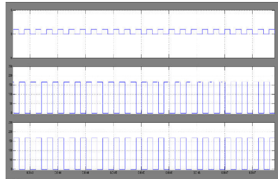
Fig.11.Simulation waveform of gate voltage (Vgs), diode Voltage (Vd4), diode Voltage (Vd3).
