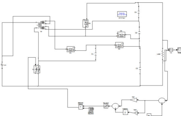
Fig.15.Matlab/simulation model of Closed loop Control of high step up Converter.
