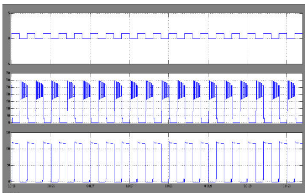
Fig.10.Simulation waveform of gate voltage (Vgs), diode Voltage (Vd2), diode Voltage (Vd2).
