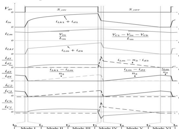
Fig. 3. Steady-state waveforms in CCM operation.
