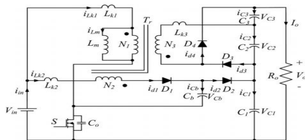
Fig. 2. Equivalent circuit of the proposed converter.
