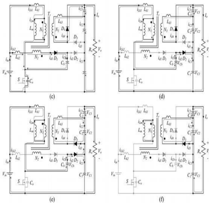
Fig. 4. CCM operating modes of the proposed converter. (a) Mode I [t0, t1]. (b) Mode II [t1, t2]. (c) Mode III [t2, t3]. (d) Mode IV [t3, t4]. (e) Mode V [t4, t5]. (f) Mode VI [t5, t6].
