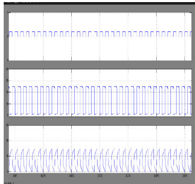
Fig.7. Simulation waveform of gate voltage (Vgs), diode Voltage (Vds), Input Current (iin).
