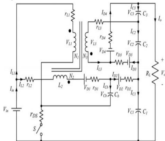
Fig. 5. Equivalent circuit including inductor conduction losses.
