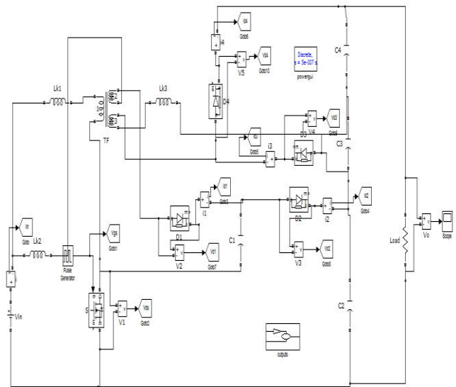
Fig.6. Matlab/simulation model of high step up Converter.
