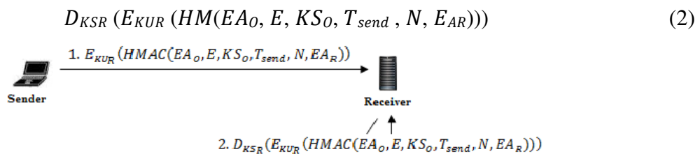
Fig.1.Authorization process of an user [1]
