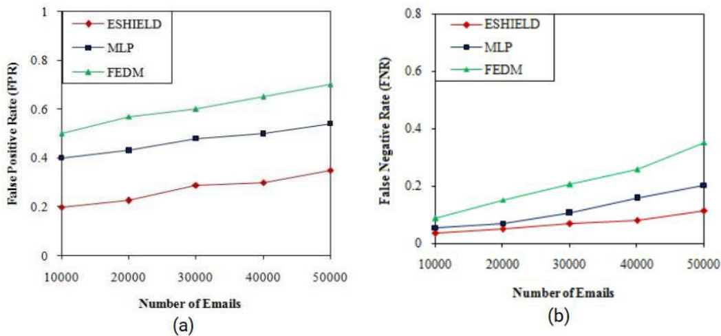
Fig.3. (a) Comparison of False Positive Rate (b) Comparison of False Negative Rate
