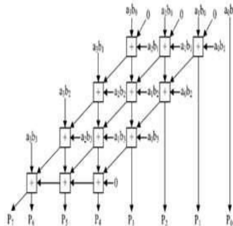
Fig. 1. 4 \times 4 normal AM.
