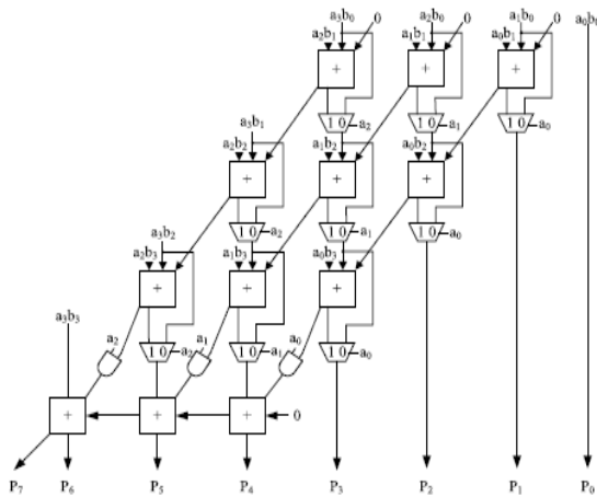
Fig. 2. 4 \times 4 column-bypassing multiplier
