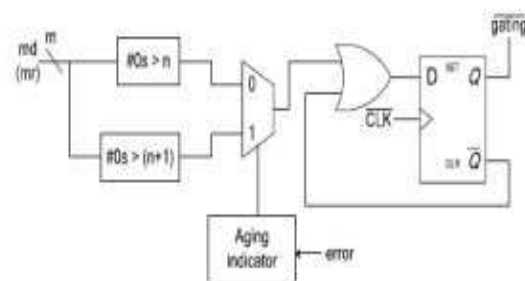
Fig. 6. Diagram of AHL (md means multiplicand; mr means multiplier).
