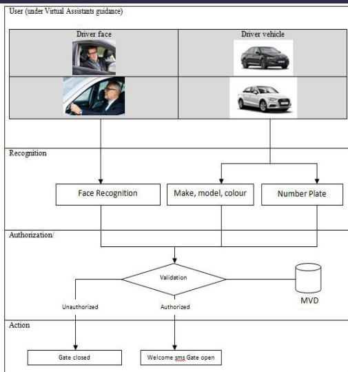
Figure 5 System Architecture of IGNS security system
