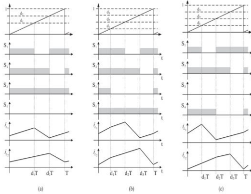
Fig. 6. Switching pattern for three states. (a) First state. (b) Second state. (c) Third state.
