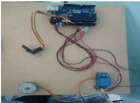
Fig6.1(a) Home section
