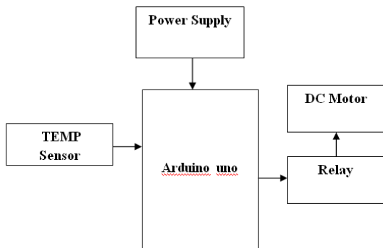
Fig 3.1:BlockDiagram of Home Section
