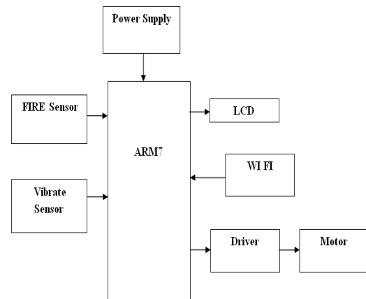
Fig3.2 :Block Diagram of Vehicle Section
