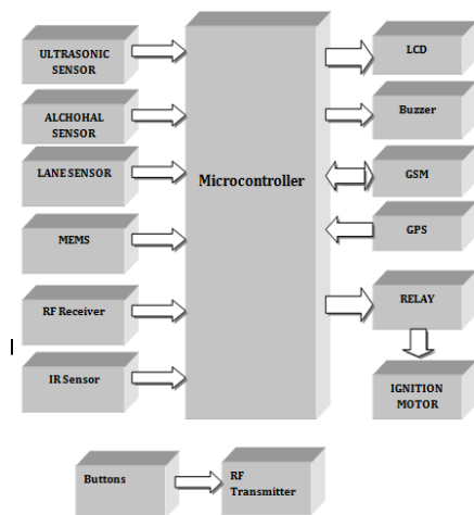
Fig 2.1:Block Diagram
