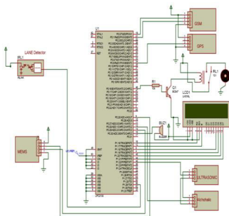
Fig 3.1:Schematic Diagram
