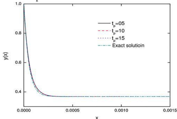
Fig. 2 Inner layer solutions for \varepsilon = 0.0001 , \delta = 0.1\varepsilon and different terminal points.
