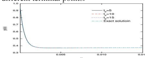
Fig. 1 Inner layer solutions for \epsilon = 0.001, \delta = 0.1\epsilon and different terminal points.
