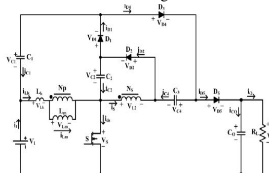
Fig. 1. Circuit configuration of the presented high step-up converter.
