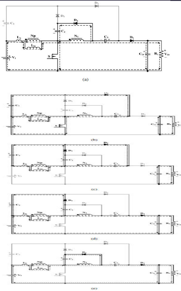
Fig. 2. Current-flow path of operating modes during one switching period at CCM operation. (a) Mode I. (b) Mode II. (c) Mode III. (d) Mode IV. (e) Mode V.
