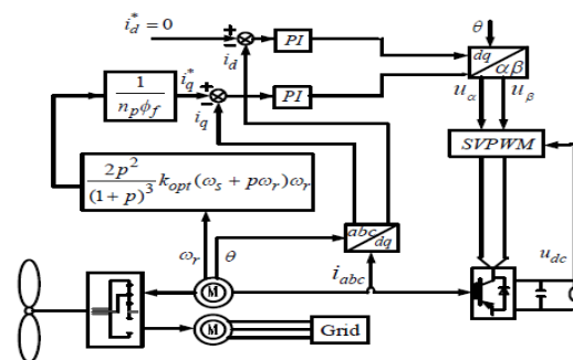
Fig.3.1. simulation model circuit.
