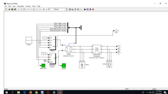
Fig.4.2. Wind power generation system.
