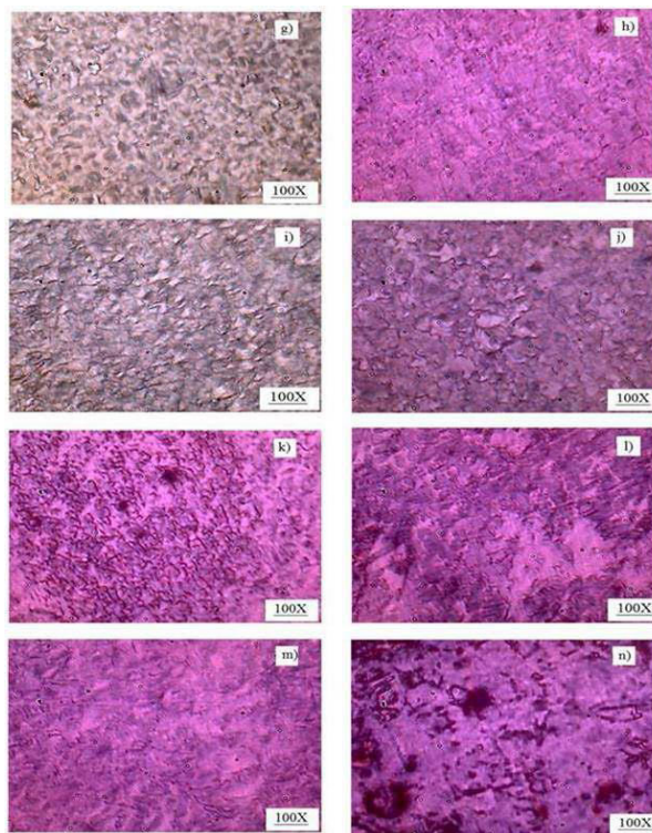
Figure 2: g) Tempered 230 air quench, h) Tempered 230 water quench, i) Tempered 350 air quench, j) Tempered 350 water quench for 8300C respectively, k) Tempered 230 air quench, l) Tempered 230 water quench, m) Tempered 350 air quench, n) Tempered 350 water quench for 8700C respectively are tempered microstructures for 0.26% C steel showing tempered martensite.
