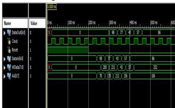
Fig 5. Encoder output
