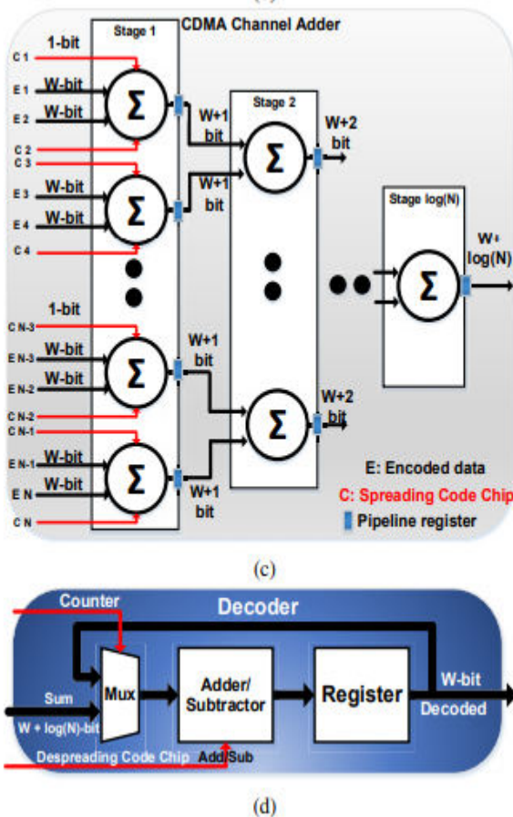
Figure 2. (c) ACDMA channel adder, (d)ACDMA decoder
