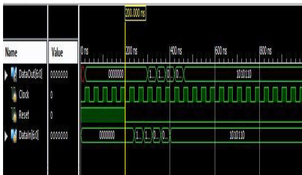
Fig 6. Decoder output
