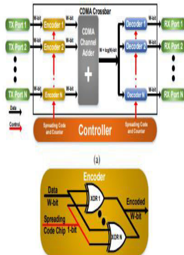
Figure 2. (a) ACDMA crossbar high-level architecture
