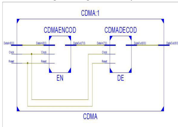
Fig 4. RTL Schematic
