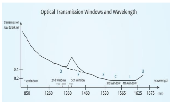
Figure.3: Optical Transmission Windows and wavelength
