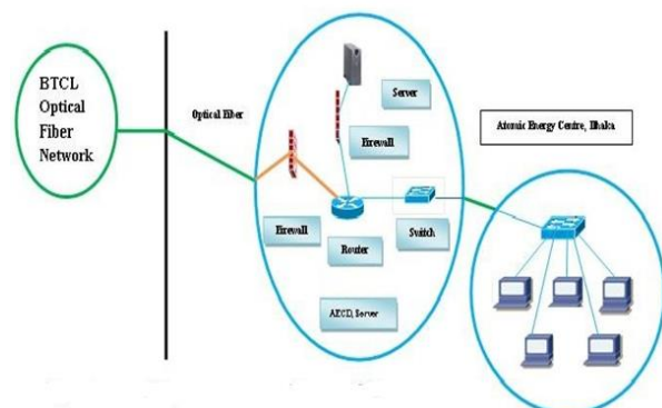
Figure.4: Diagram of Optical Fiber network at AECD
