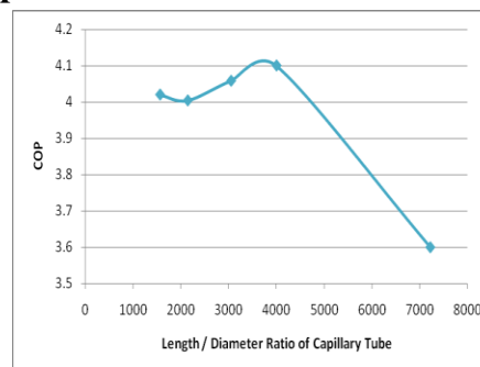
Graph.1 Effect of L/D of capillary tube on coefficient of performance
