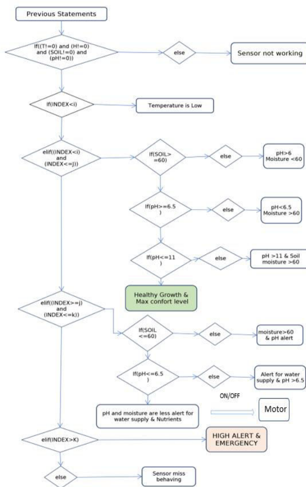
Fig 8: Flowchart
