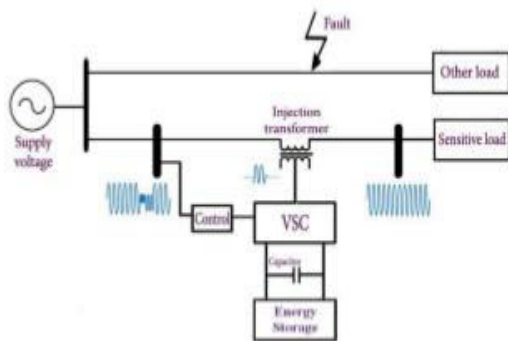
Figure (2) Basic DVR topology
