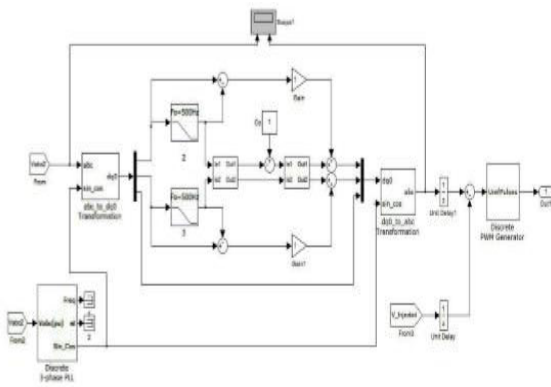
Figure (6) Block diagram control scheme of DVR
