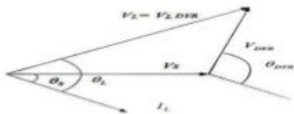
Figure (3) phasor diagram of pre-sag/dip method
