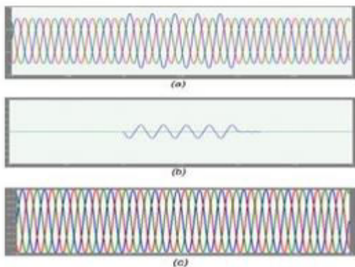
Figure 11 – Single phase voltage swell : a) Source Voltage b) Injected Voltage , c) Load Voltage
