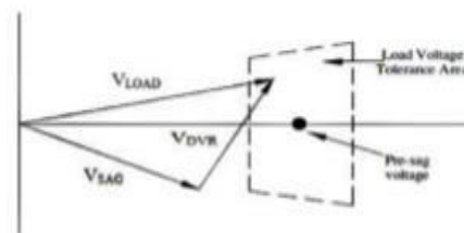
Figure (5) voltage tolerance method with minimum energy injection
