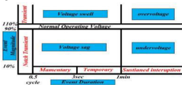
Figure (1) Voltage reduction standard of IEEE 1159-1995
