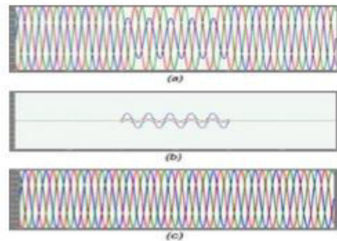
Figure 9 - Single phase voltage sag : a) Source Voltage b) Injected Voltage , c) Load Voltage
