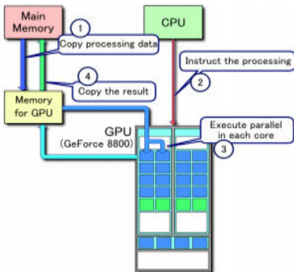
Fig 3: Processing Flow between GPU and CPU
