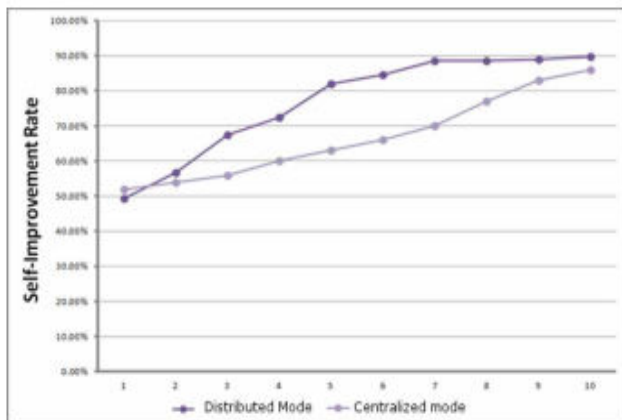
Figure 5. Comparison of self-improvement rate and centralized mode
