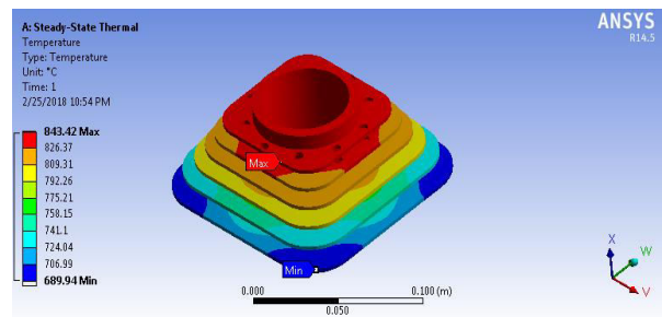
Figure 14 Temperature distribution on al2014
