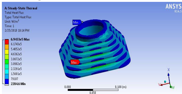
FIGURE 25 HEAT FLUX IN GREY CAST IRON
