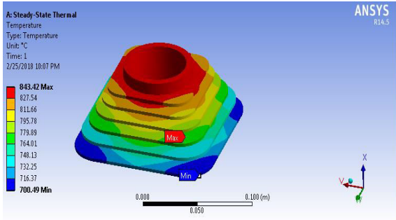
Figure 17 Temperature distribution on al2014
