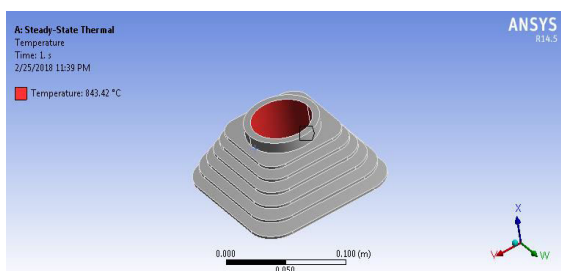
Figure 11 Temperature of boundary conditions and without holes
