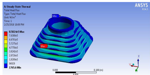
Figure 23 Heat flux on al2014
