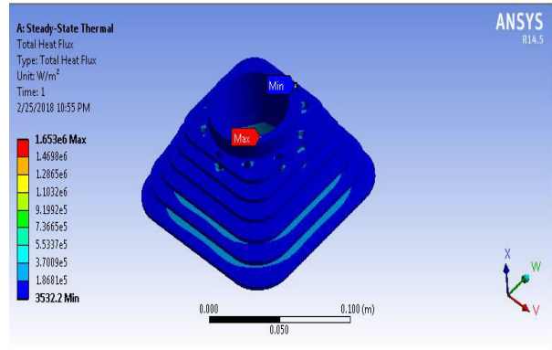
Figure 20 Heat flux on al2014.
