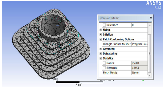
Figure 8 Mesh with holes
