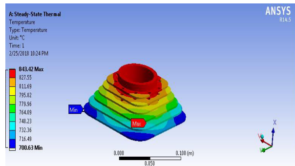
Figure 15 Temperature distribution on Al6061
