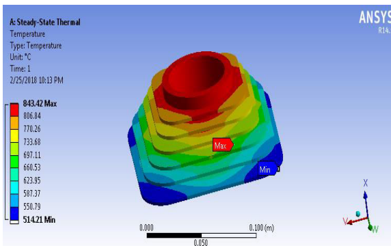
Figure 19 Temperature distribution on grey cast iron
