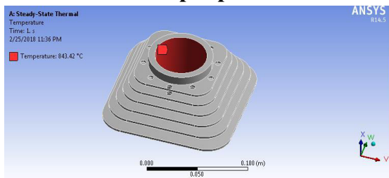
Figure 10 Temperature of boundary conditions with holes
