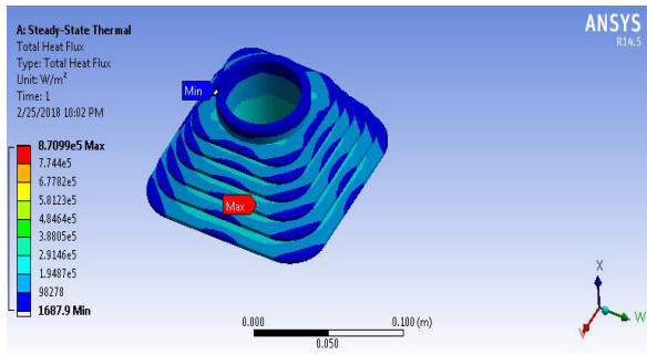
Figure 24 Heat flux in al6061
