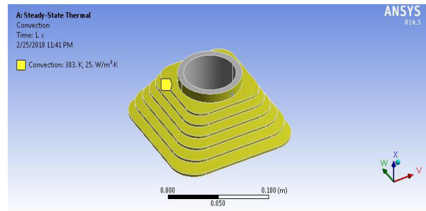
Figure 13 Convection of boundary conditions with out holes
