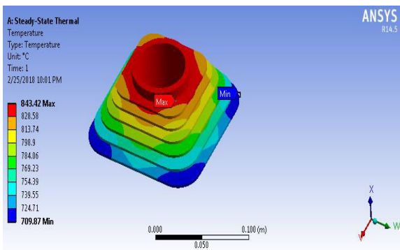
Figure 18 Temperature distribution on al6061
