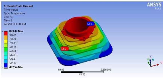
Figure 16 Temperature distribution on grey cast iron
