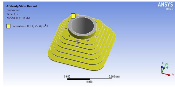
Figure 12 Convection of boundary conditions with holes
