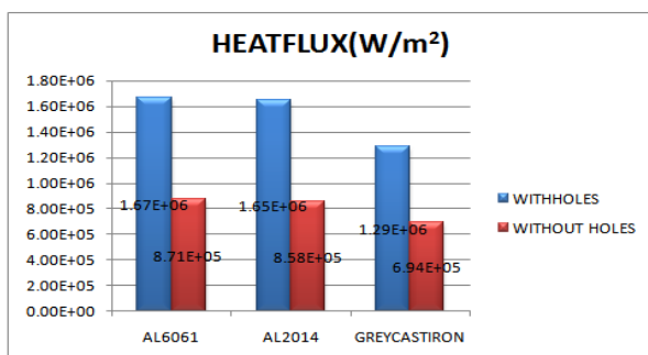
FIGURE 27 TOTAL HEATFLUX WITH AND WITHOUT HOLES
