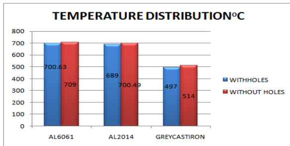
FIGURE 26 WITH HOLES AND WITHOUT HOLES TEMPERATURE DISTRIBUTION OF CYLINDER FINS
