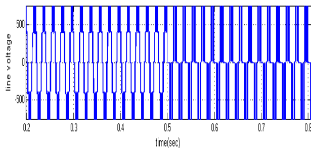
Fig.13. Simulated wave form of Line Voltage of the Inverter at MI=1 with Diode short fault.
