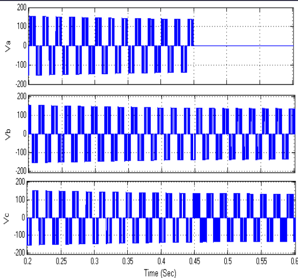
Fig.40. Simulated wave form of Phase voltage of the Inverter at MI=1 with Switch Short fault.
