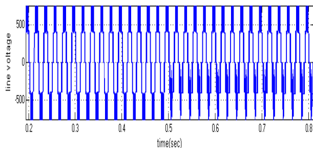
Fig.25. Simulated wave form of Line Voltage of the Inverter
