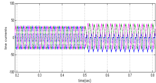
Fig.26. Simulated wave form of Line Current of the Inverter at MI=1 with Switch open fault.
