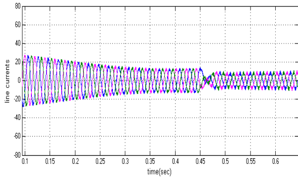
Fig.35. Simulated wave form of Line Current of the Inverter at MI=1 with Switch open fault.
