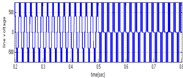
Fig.29. Simulated wave form of Line Voltage of the Inverter at MI=1 with Switch short fault.
