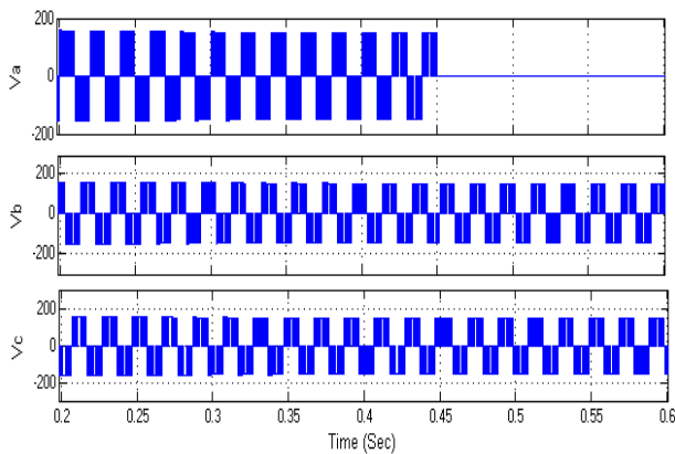
Fig.36. Simulated wave form of Phase voltage of the Inverter at MI=1 with Switch open fault.
