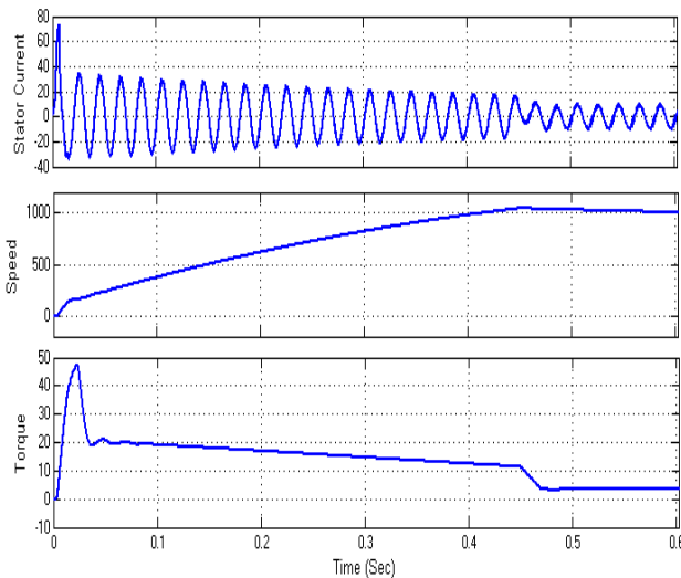
Fig.41. Performance characteristics of Current, Speed and Torque at MI=1 with Switch Short fault.
