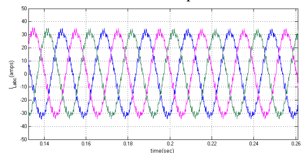
Fig.10. Simulated wave form of Line Current of the Inverter at
