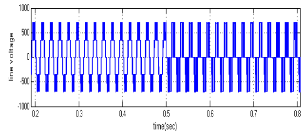
Fig.21. Simulated wave form of Line Voltage of the Inverter at MI=1 with Gate short fault.
