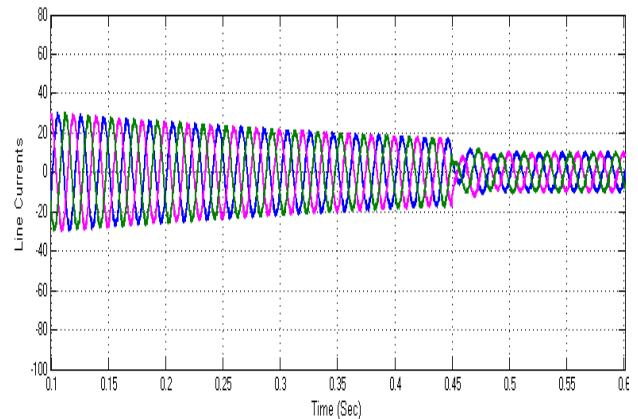
Fig.39. Simulated wave form of Line Current of the Inverter at MI=1 with Switch Short fault.
