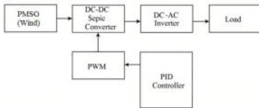
Fig.1.1. Basic model
