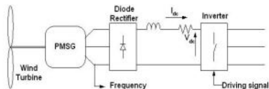
Fig.3.2. Proposed model.
