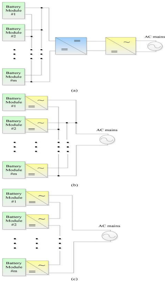
Fig.2. Different configuration of the battery energy storage system.(a) Two-stage configuration. (b) Micro inverter configuration.(c) Cascade-type configuration.
