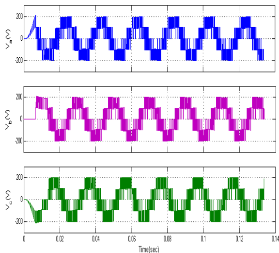
Fig.19 Line-Line Voltages of MLI
