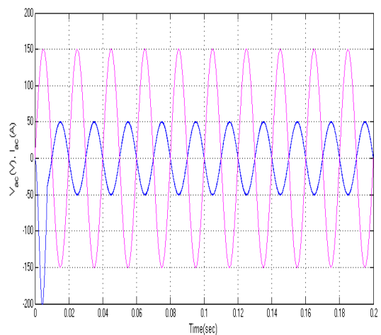
Fig.17 Ac main Voltage and Output current for BSG-Inverter in charging mode
