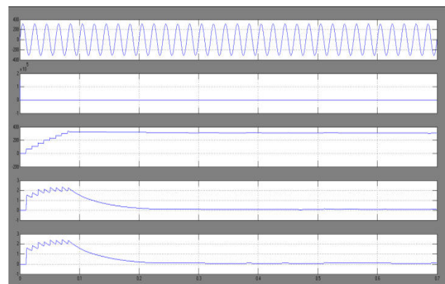
Fig 7 simulation wave form of Input voltage, current, buck-boost converter output voltage, half bridge VSI output voltages, and currents at 220 V and full load.
