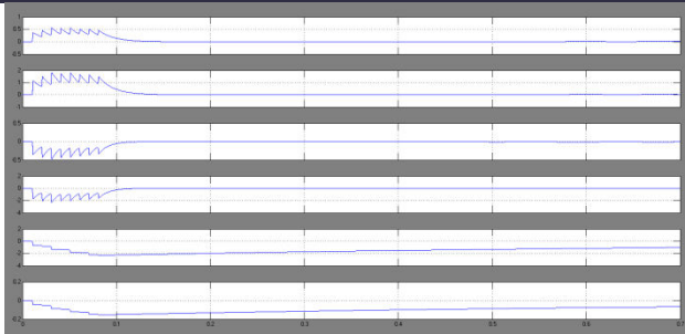
Fig 8 simulation wave form of Input voltage, current, bridgeless buck boost converter output voltage, half-bridge VSI output voltages, and currents at load variation in +12- and +5-V outputs at 0.25 s.
