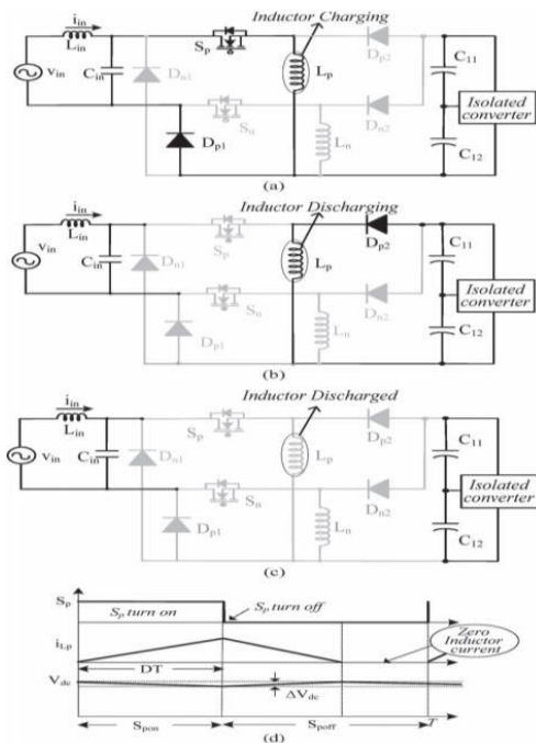
Fig.2. Operating modes for under (a) upper switch S_p is on, (b) upper switch S_p is off, (c) both switch and diode are off, and (d) waveforms in one switching cycle.
