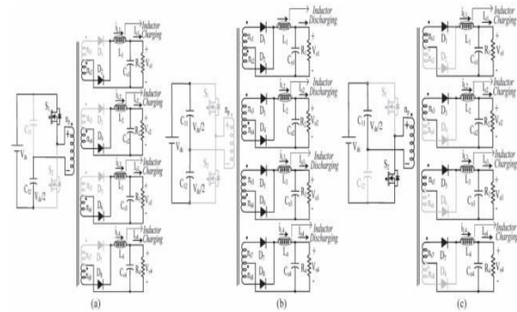
Fig.3. (a) When the first switch S_1 is on, (b) when both switches are off, (c) and when the second switch S_2 is on.
