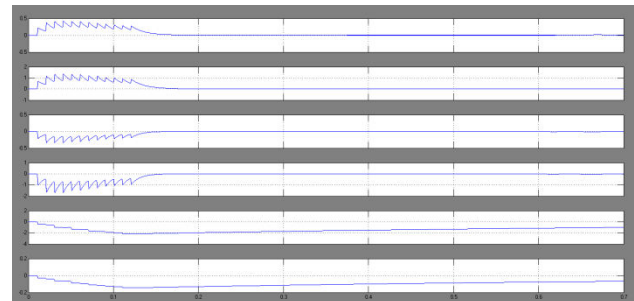
Fig 12 simulation wave form of Input voltage, current, bridgeless buck boost converter output voltage, half-bridge VSI output voltages, and currents at load variation in +12- and +5-V outputs at 0.25 s with variable load
