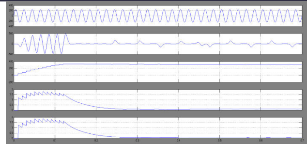
Fig 11 simulation wave form of Input voltage, current, buck-boost converter output voltage, half bridge VSI output voltages, and currents at 220 V and full load with variable load
