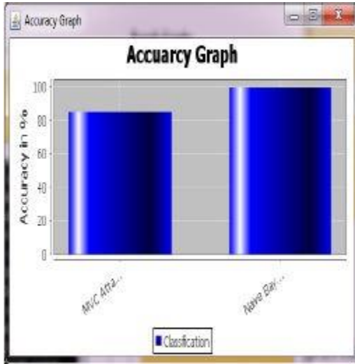
Figure 3. Accuracy Graph
