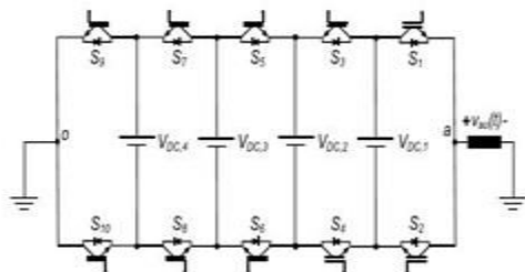
Fig.12. PUC MLI topology as proposed
