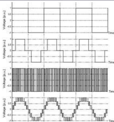
Fig.1. Typical inverter waveforms: (a) Square wave. (b) Quasi-square wave. (c) Two-level PWM waveform. (d) Multilevel PWM waveform.
