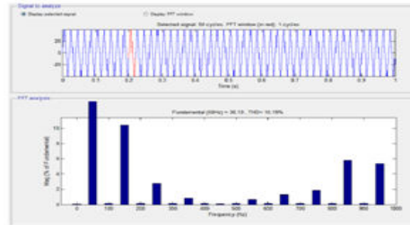
Fig.18 AC Inverter output THD
