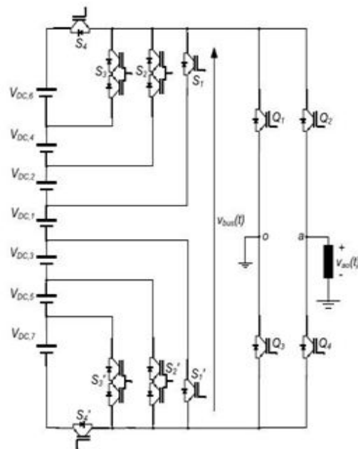
Fig.15. 2SELG-based MLI as proposed
