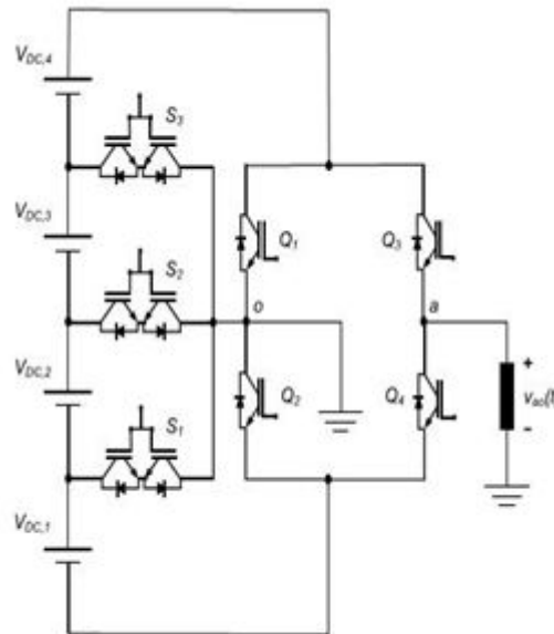
Fig.8. T-type inverter as proposed
