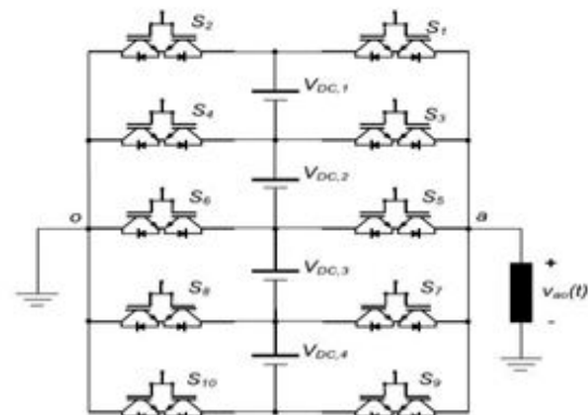
Fig.11. CBSC-basedMLI as proposed
