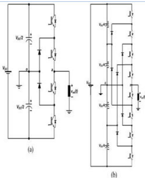
Fig.3. One leg of neutral-point / diode-clamped structure; (a) three-level; and (b) five-level.
