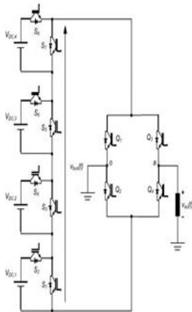
Fig.7 Cascaded half-bridge-based MLDC inverter as proposed.
