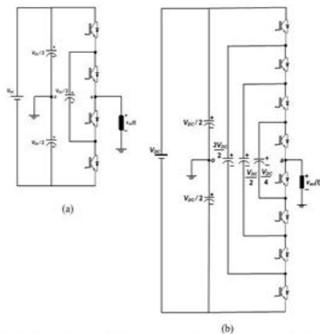
Fig.4. One leg of flying capacitor structure: (a) three-level; and (b) five-level.
