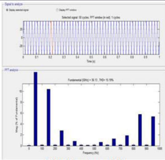
Fig.22 AC Inverter output THD
