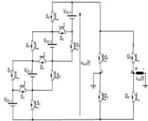
Fig.9. SSPS-based MLI as proposed
