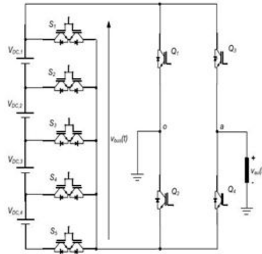
Fig 13. MLM-based MLI as proposed
