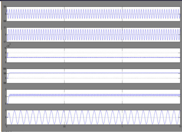
Fig 17 simulation wave form of proposed converter of source voltage, source current, dc link voltage, speed, torque and stator currents
