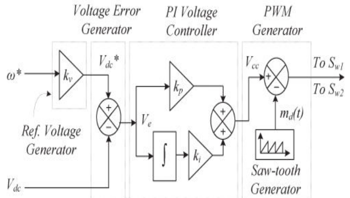
Fig. 5. PI Control of the PFC BL-CSC converter feeding BLDC motor drive.
