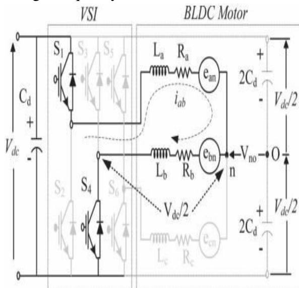
Fig. 6. Three-phase VSI feeding a BLDC motor.
