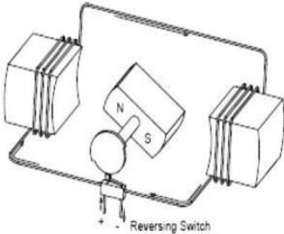
Fig.1 Basic operation of BLDC Motor.
