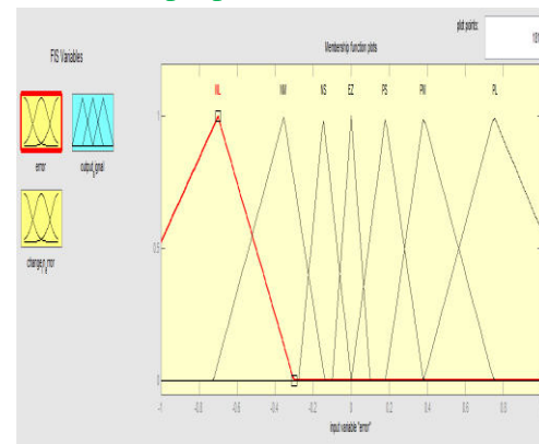
Fig.9. Membership functions for error.
