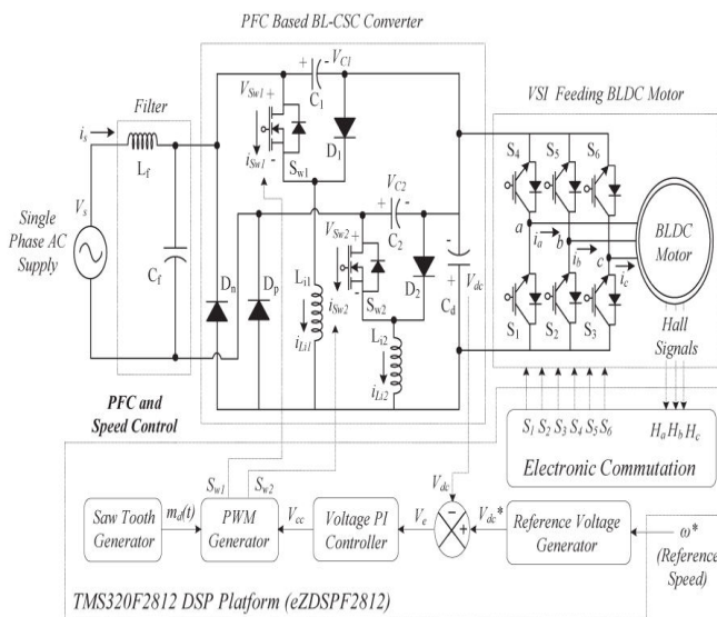
Fig.3. Proposed BL-CSC converter-fed BLDC motor drive.
