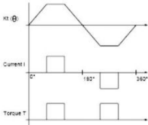
Fig.2 Waveform of current and torque.
