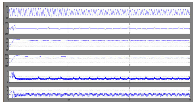
Fig 15 simulation wave form of conventional converter of source voltage, source current, dc link voltage, speed, torque and stator currents during sudden change in supply voltage
