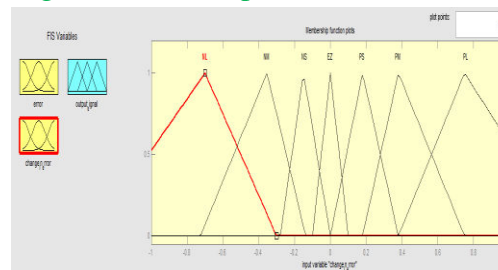
Fig.10. Membership functions for change_in_error.
