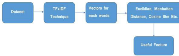
Fig. 2: TF-IDF block diagram.
