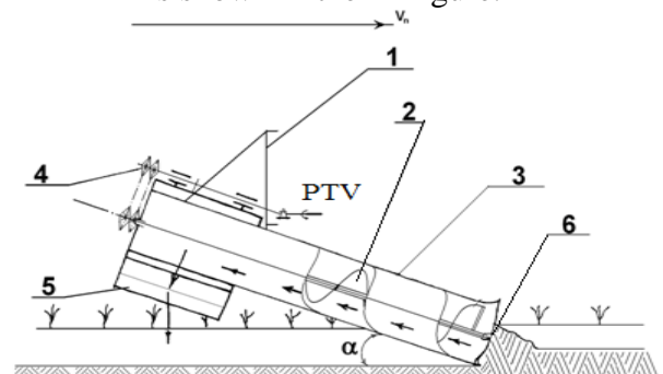
Figure 1. Pawl-creating device between cotton rows
