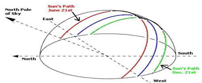
Fig. 1: Sun's apparent motion.
