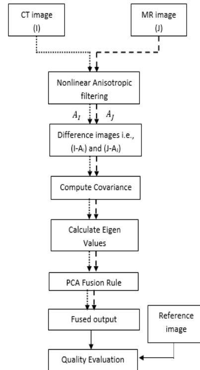
Fig. 3: Proposed NLAFF-PCA fusion process flow.
