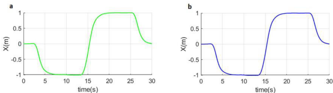
Fig. 11 X position of quadcopter over time. (a) with wind disturbances. (b) without wind disturbances
