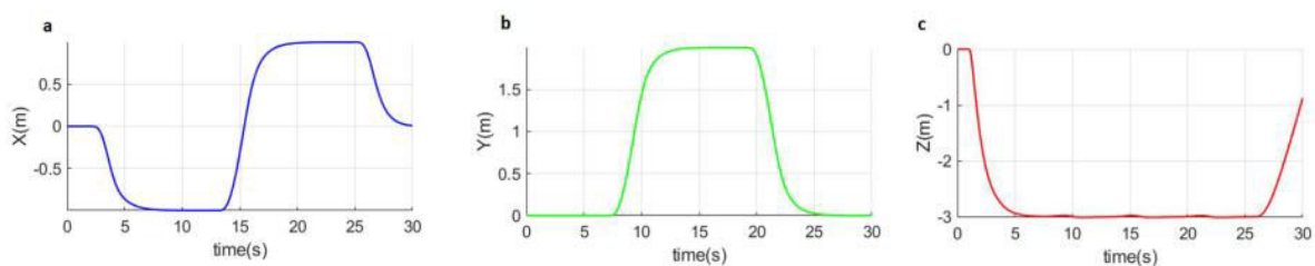
Fig. 9 Quadcopter change in position over time for LQR controller. (a) X position over time. (b) Y position over time. (c) Z position over time
