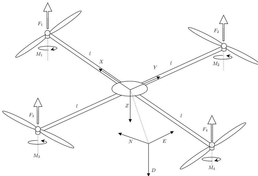
Fig. 1 Quadcopter system illustration with its relative coordinate systems
