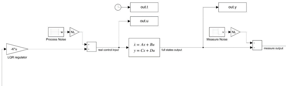
Fig. 4 LQR controller quadcopter system architecture
