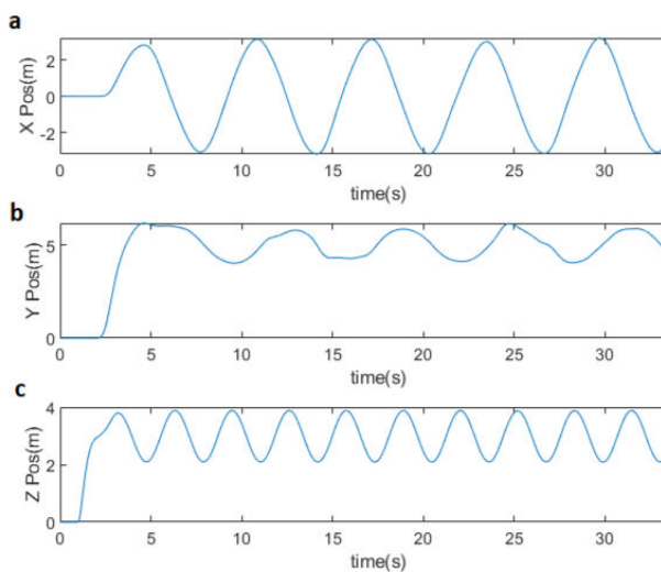
Fig. 6 Quadcopter change in position over time for PID controller. (a) X position over time. (b) Y position over time. (c) Z position over time
