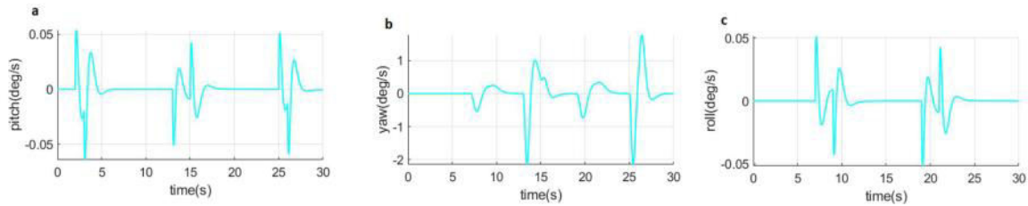
Fig. 10 Quadcopter angular rates over time for LQR controller. (a) pitch over time. (b) yaw over time. (c) roll over time
