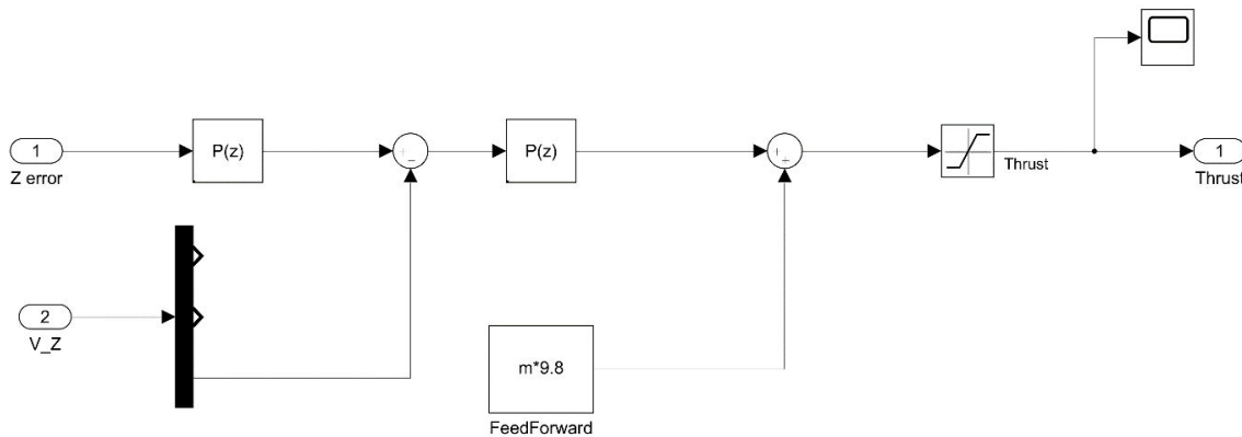
Fig. 2 Thrust controller block diagram
