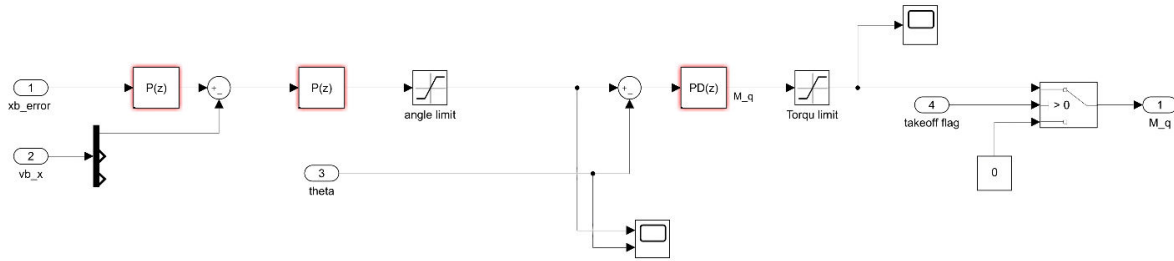
Fig. 3 Pitch controller block diagram
