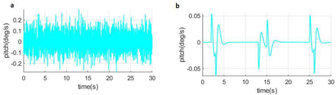
Fig. 12 Pitch angle of quadcopter over time. (a) with wind disturbances. (b) without wind disturbances
