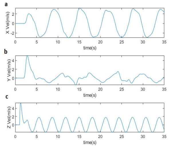
Fig. 7 Quadcopter change in velocity over time. (a) X velocity over time. (b) Y velocity over time. (c) Z velocity over time
