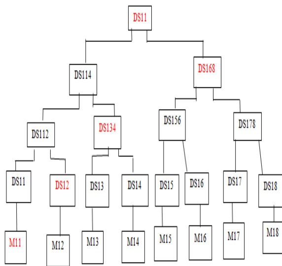
Fig-1: Process of hash tree generation Process of hash generation in sender side
