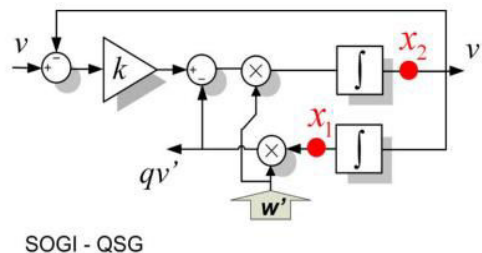
Fig.10. Quadrature signal generator based on a second order generalized integrator (SOGI QSG).
