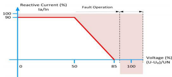
Fig.5. REE voltage support requirement in the event of grid fault.
