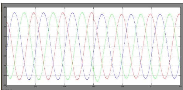
Fig.16 simulation wave form DSOGPLL harmonic, frequency, LLLG and unbalance condition
