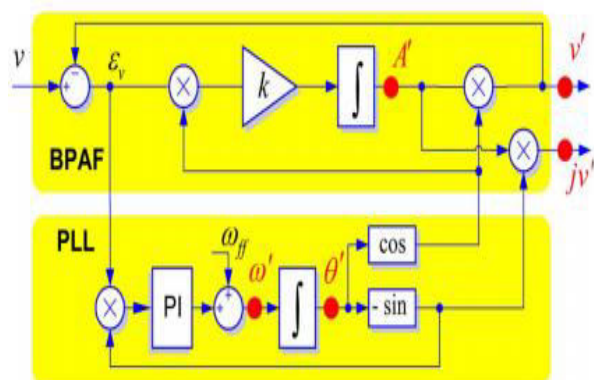
Fig.12. Quadrature signal generator based on an EPLL structure
