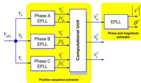
Fig.8. 3phEPLL block diagram.
