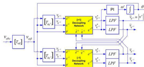
Fig.6. DDSRF-PLL block diagram.
