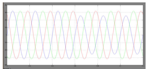
Fig 18 simulation wave form of (3phEPLL) Harmonic, frequency, LLLG and unbalance condition
