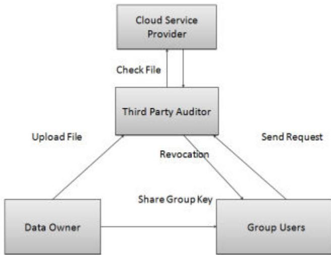
Fig. 3. Architecture of a proposed system
